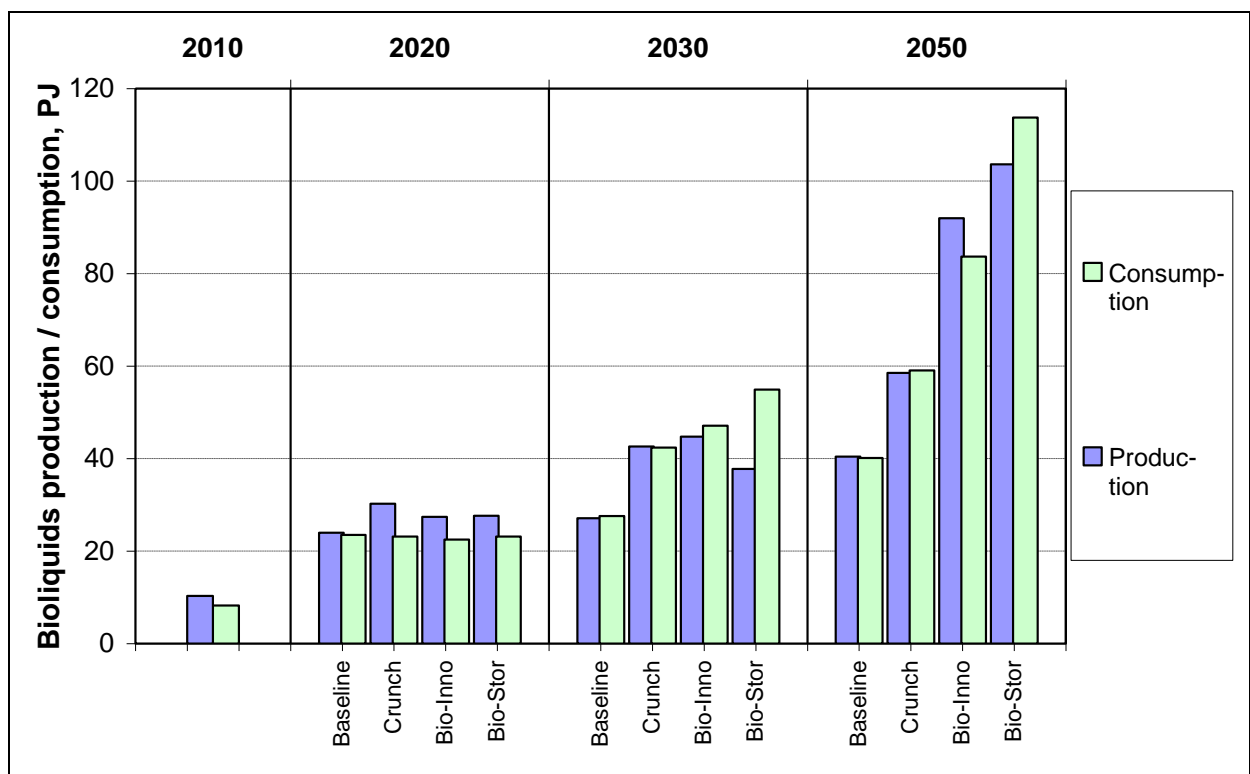
Figure 39. Demand and production of liquid biofuels in Finland.
