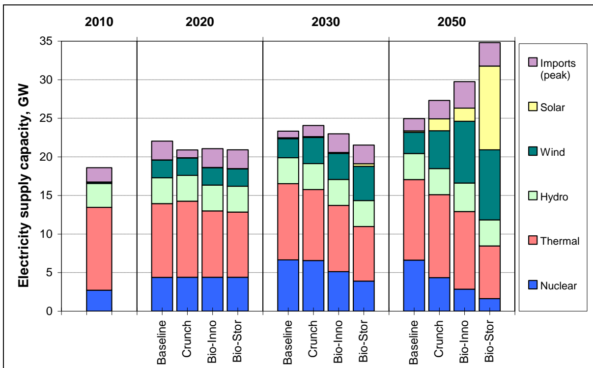
Figure 37. Development of electricity supply capacity in Finland. Imports refer to the utilized capacity during the peak.
