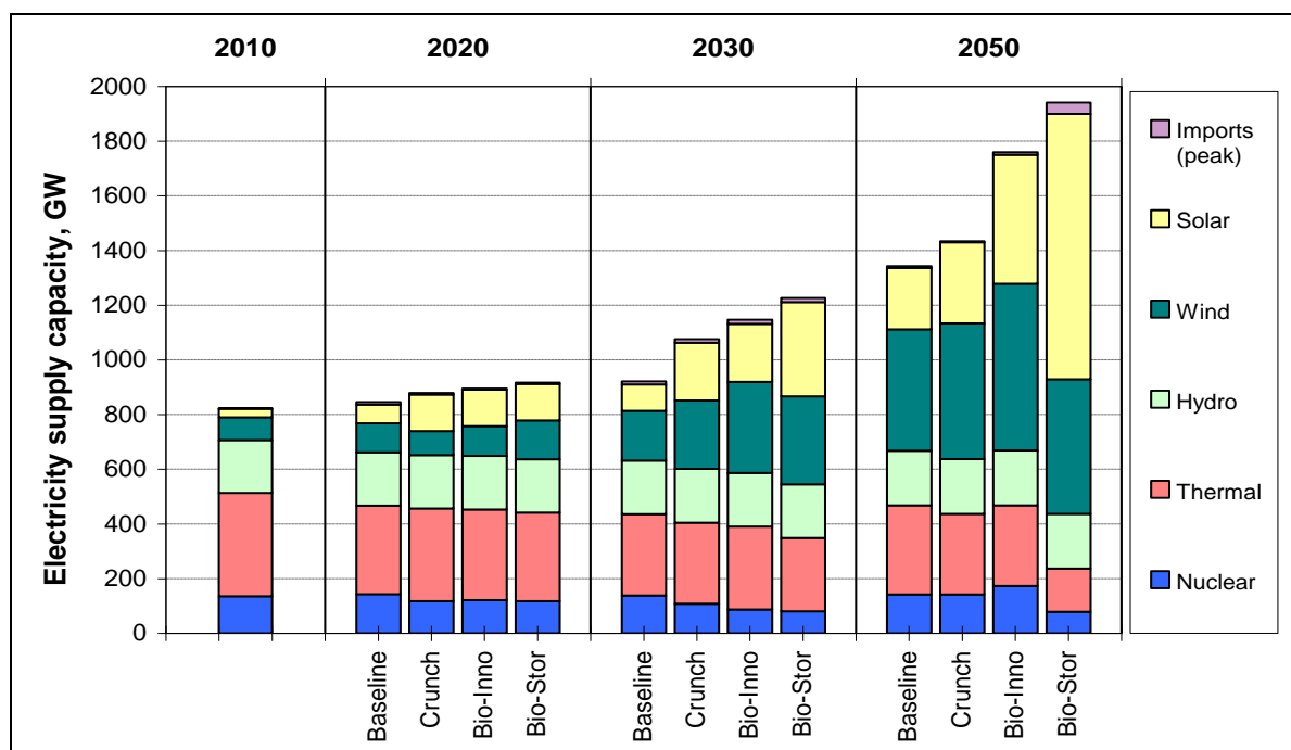
Figure 30. Development of electricity generation capacity in Europe.
