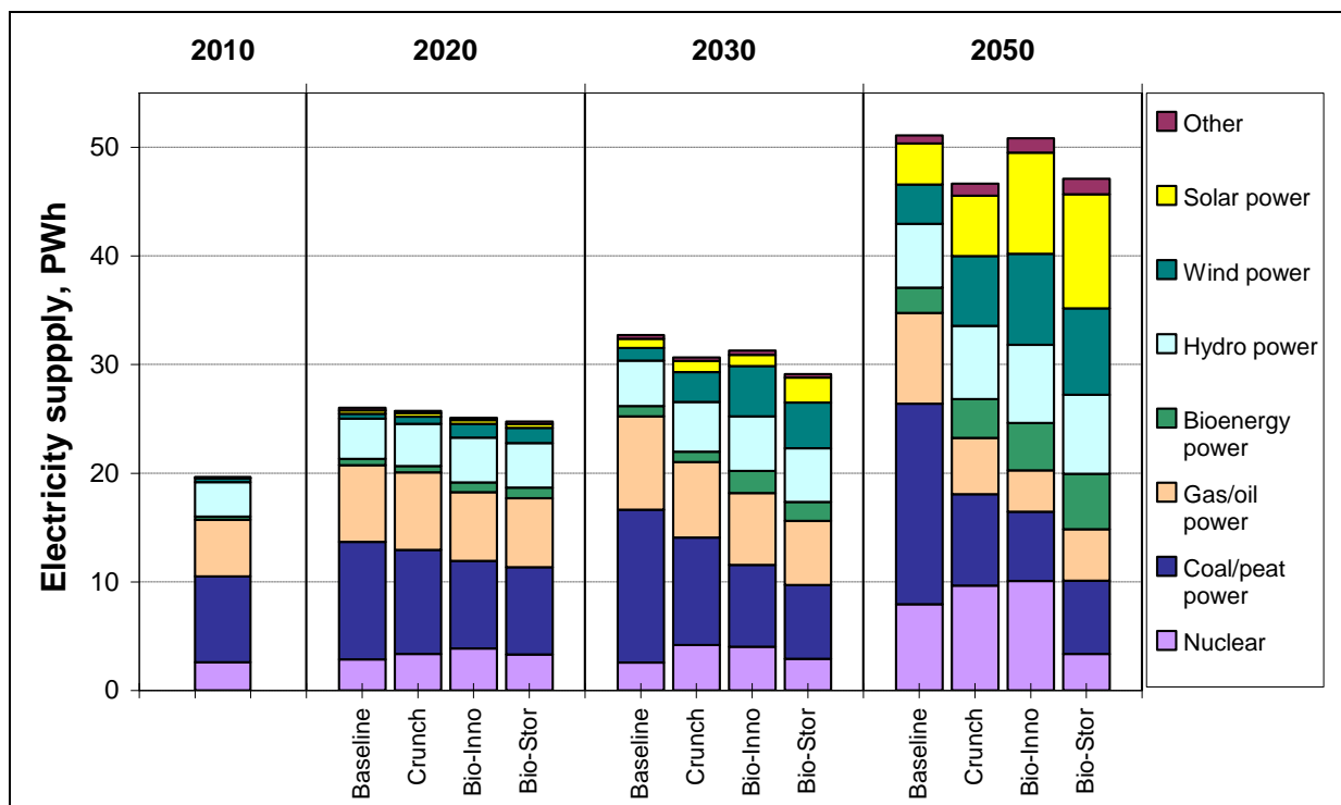
Figure 21. Global total electricity generation.
