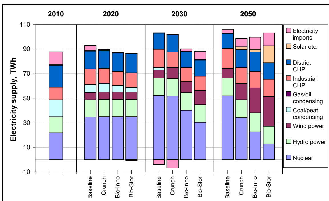
Figure 35. Development of electricity supply in Finland.
